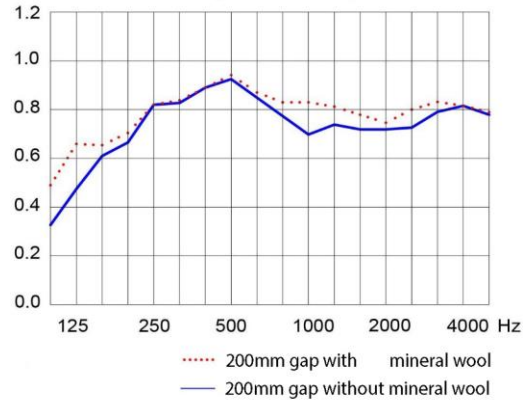
Absorption according to EN ISO 354
